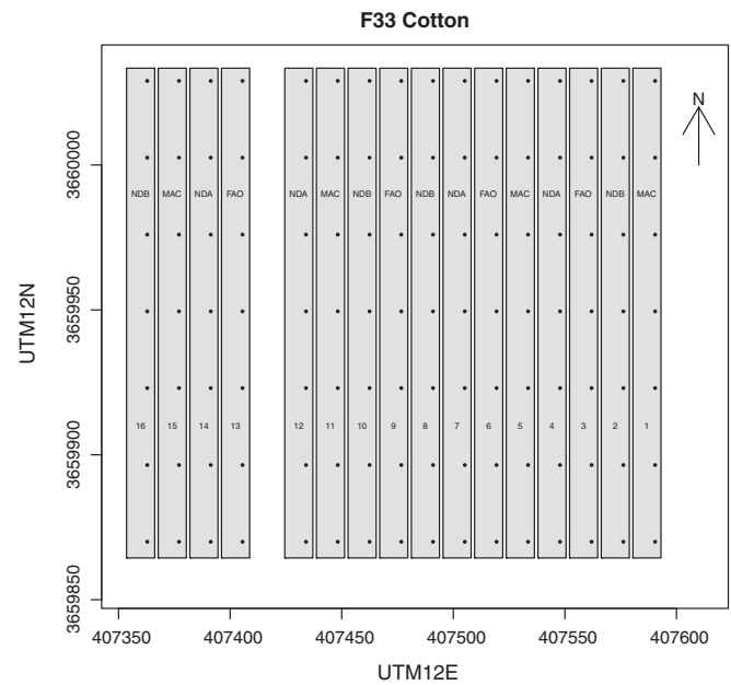
Fig. 1. Experimental layout for cotton grown at Maricopa, Arizona in 2009 and in 2011. Numbers denote plot identifiers, codes indicate their corresponding irrigation treatment type, dots indicate location of neutron probe access tubes ( 7 \times 16 ) for soil moisture monitoring.
