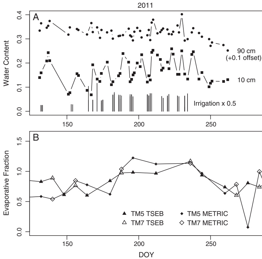
Fig. 11. Testing remote sensing detection of crop water stress. Soil moisture content at two depths (A) and EF derived from TSEB and METRIC for 2011 observations (B) are plotted for the entire cotton growing season.
