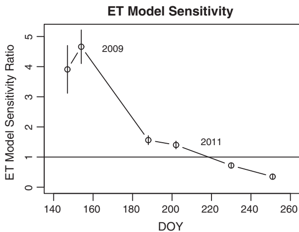
Fig. 4. Daily ET model sensitivity over cotton. Slopes derived from fits shown in Fig. 3 are plotted vs. time to show the decreasing relative sensitivity of METRIC estimates to TSEB estimates. At DOY 220, model sensitivities are approximately equal.
