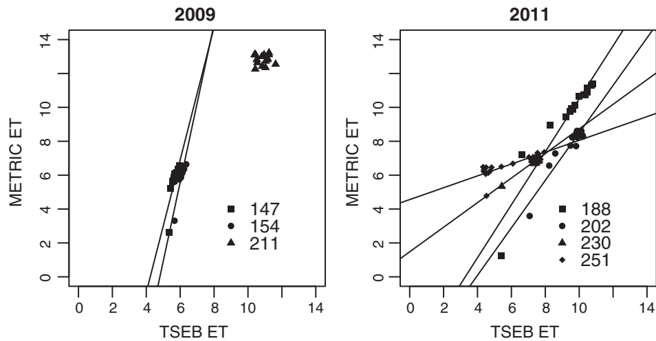
Fig. 3. Daily ET from TSEB and METRIC compared for 2009 and 2011. Each symbol represents one of 7 particular days. The lines are linear models representing the relative model sensitivities of ET over cotton canopy. No linear fit was created for DOY 211 due to lack of linear trend.
