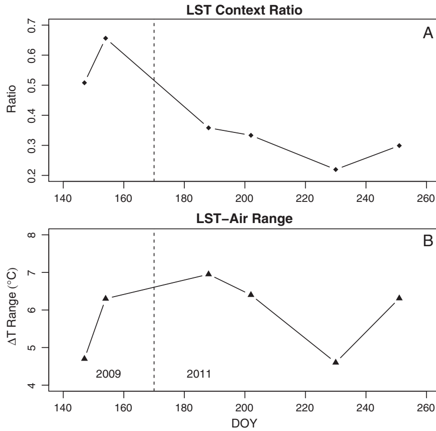
Fig. 5. Factors controlling ET model sensitivity. METRIC ET values are determined by scaling LST observations with respect to cold and hot pixels; its sensitivity of ET estimates to LST changes is controlled by the relative range of vegetation LSTs to the range spanned by cold to hot reference pixels. Shown are ratios between these ranges for the different airborne flight days (A). TSEB ET values, on the other hand, are controlled by LST/air temperature differences ( \Delta T ) and do not use reference pixels. Thus where for sites with a nearly constant air temperature, TSEB model sensitivity is controlled by absolute vegetation LST (B). The dashed line separates 2009 and 2011 data.
