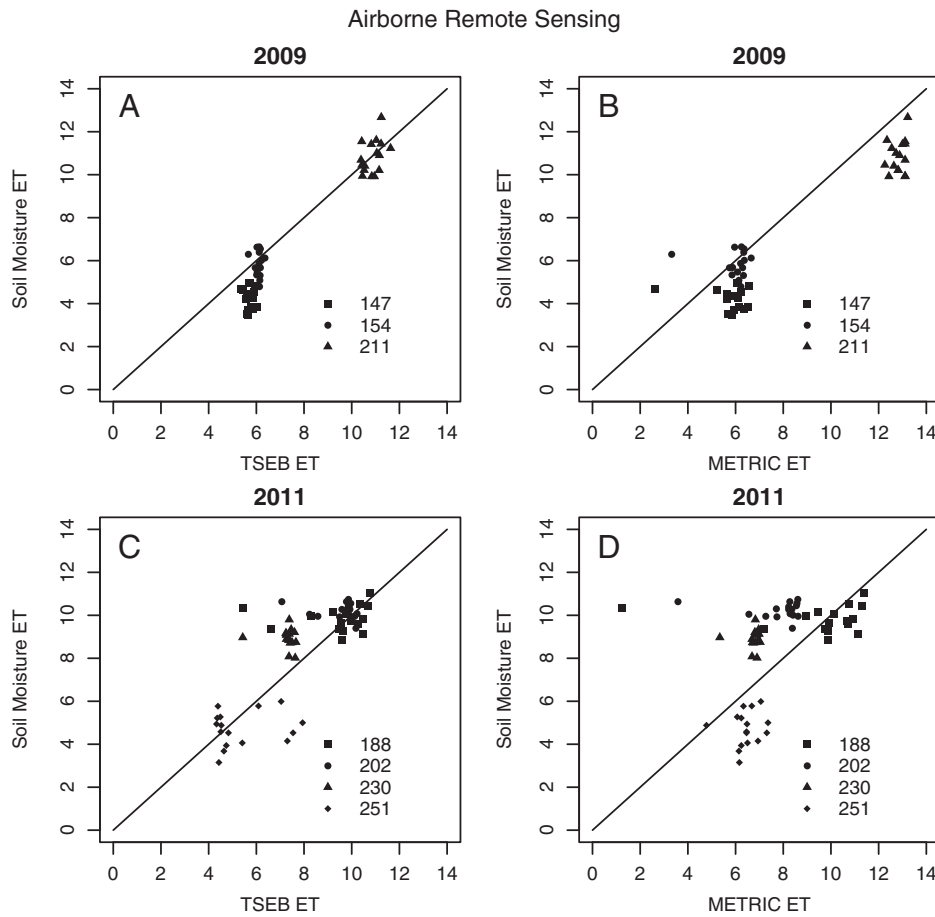
Fig. 2. Modeled and reference daily ET derived from airborne remote sensing in 2009 and 2011. Border-averaged ET estimated with TSEB (left column) and METRIC (right column) are compared with soil moisture derived ET.
