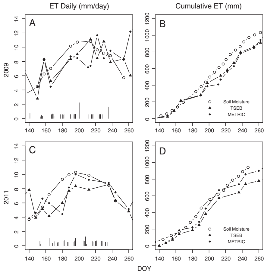
Fig. 10. Landsat-derived daily and cumulative ET for 2009 and 2011 using TSEB and METRIC.
